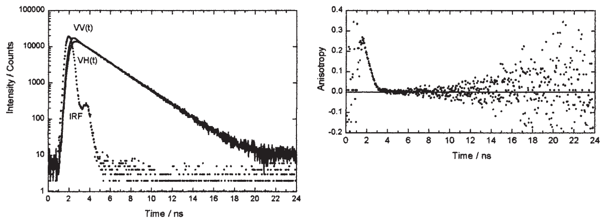
Fig. 4. VV and VH polarized decays of Coumarin 6 in dimethyl sulfoxide and the instrument response function. The anisotropy decay curves calculated from VV(t) and VH(t) directly, is plotted at right panel.
