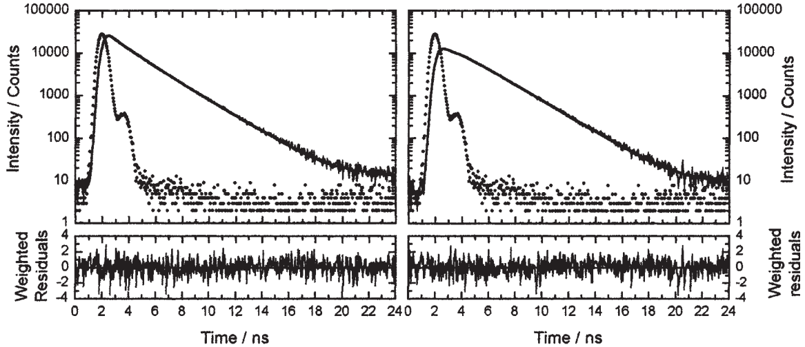
Fig. 3. Double-exponential reconvolution analyses of VV (at left) and VH (at right) polarized decays of Coumarin 6 in ethylene glycol.
